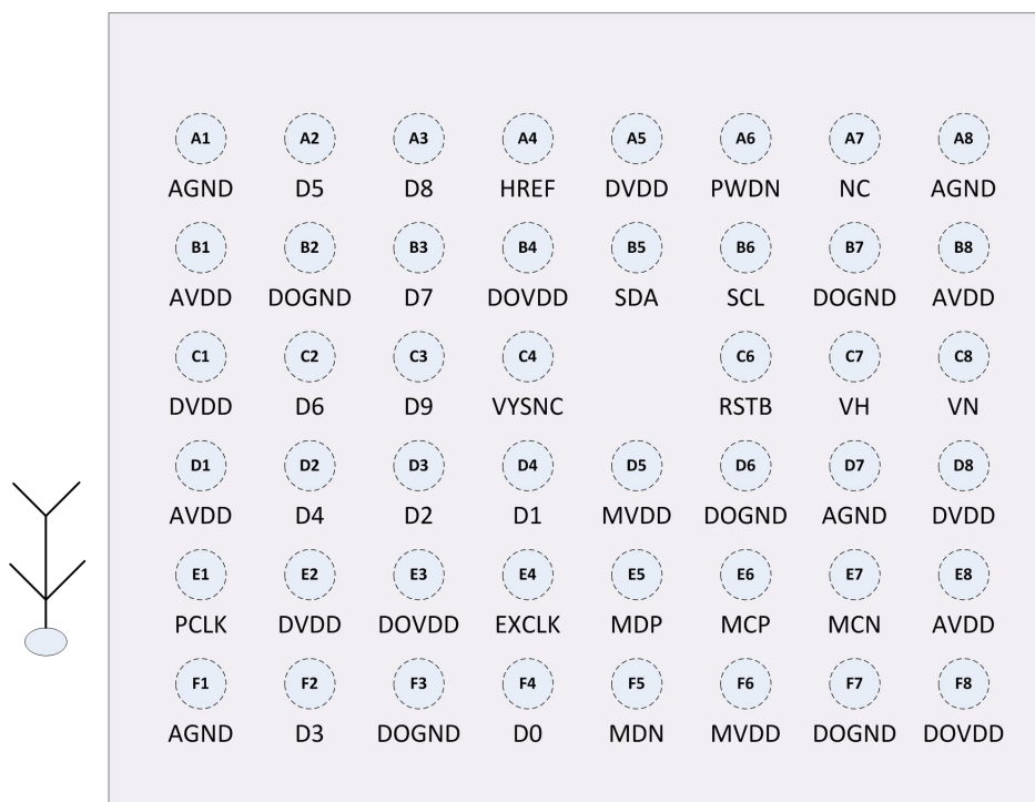
Figure 1: JX-H65 CSP top view
