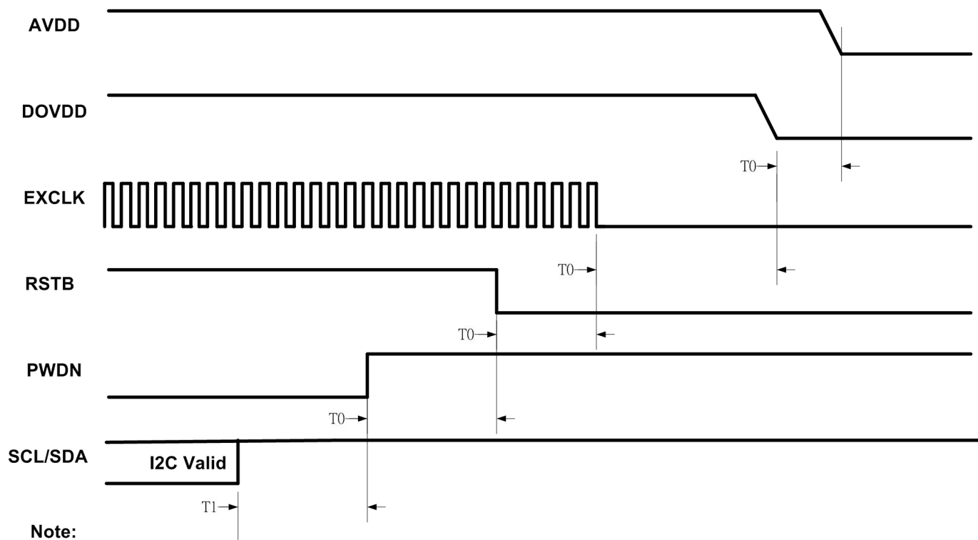
Figure 13. Power down sequence for JX-H65
