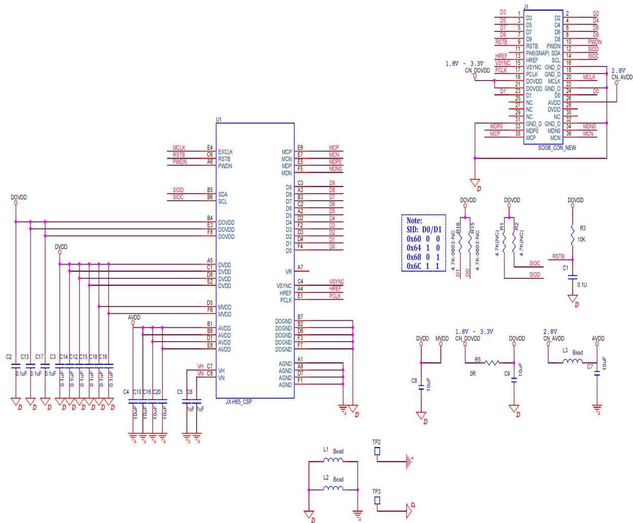
Figure 16. Reference schematic for CSP module
