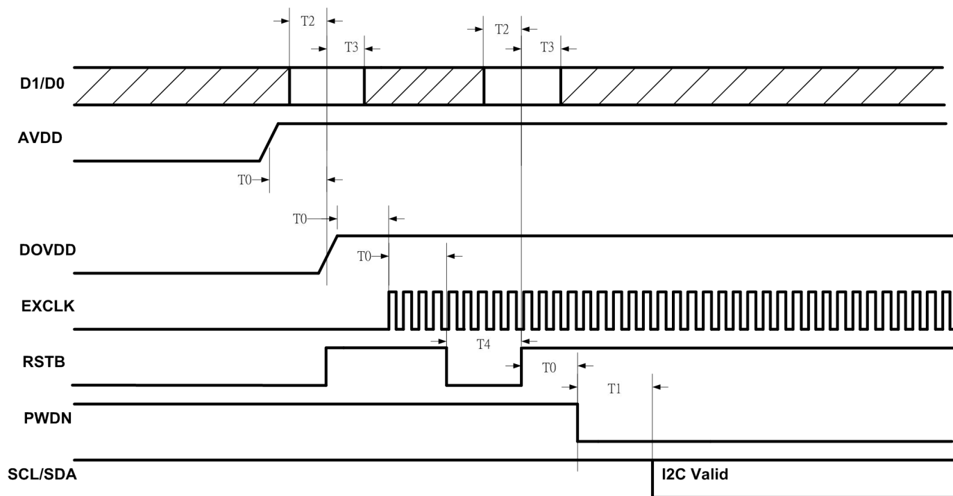
Figure 12. Power up sequence for JX-H65
