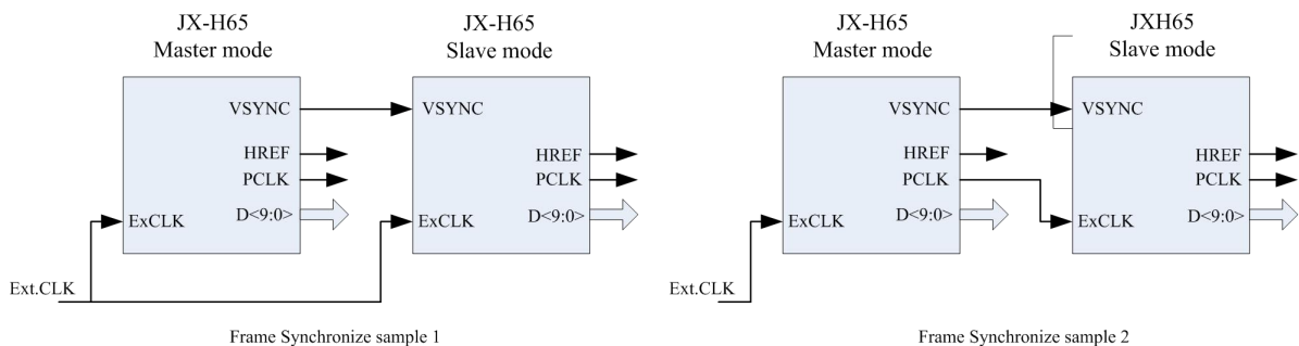
Figure 10: Frame Synchronization illustration
