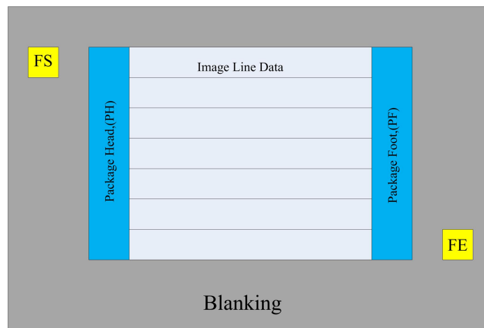
Figure 9: MIPI interface frame timing
