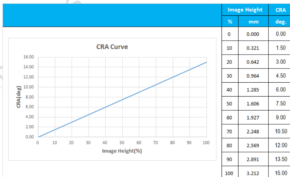
图 4-2 CRA Curve
