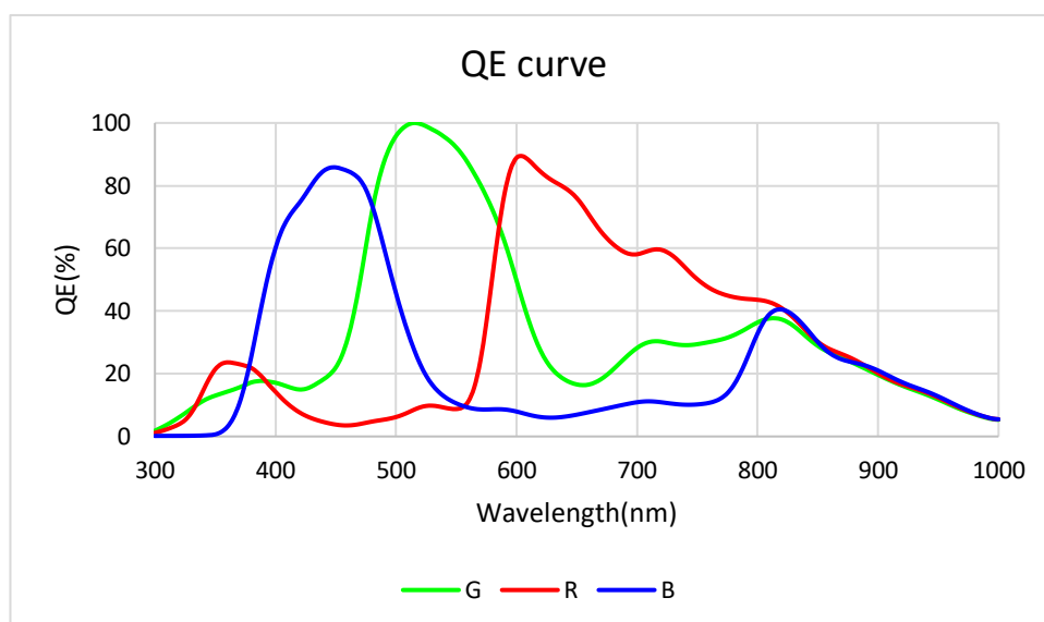
图 4-1 QE Curve
